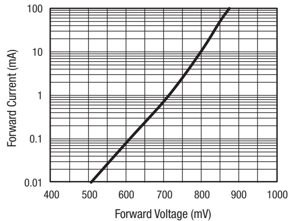
Figure 2. DC Characteristics
