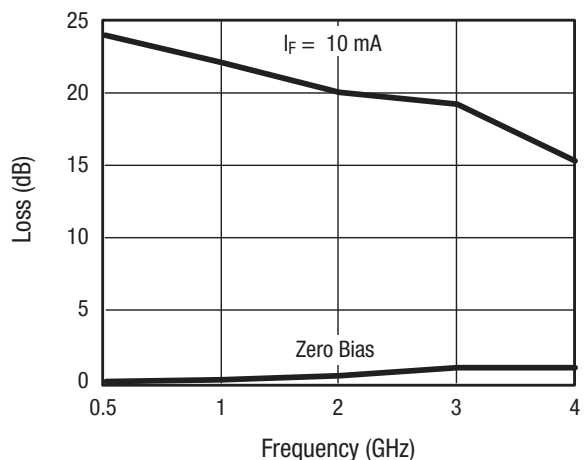
Figure 5. SMP1322-017 Typical SPST Switch Performance
