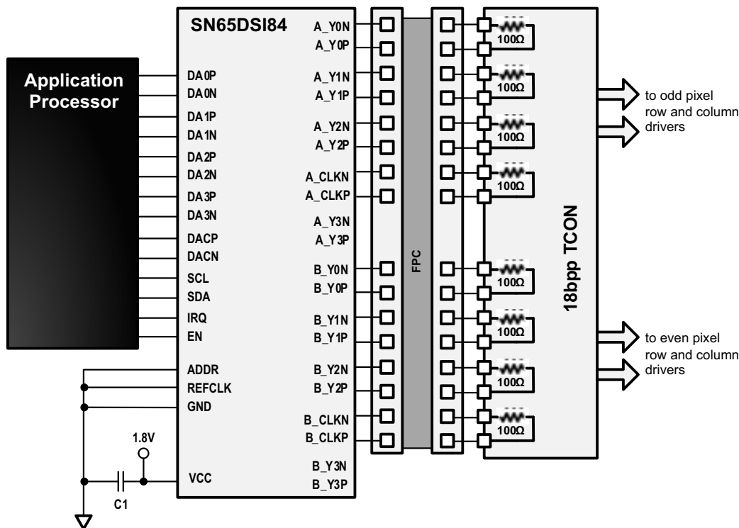
Figure 19. Typical 1920 x 1200 WUXGA 18-bpp Panel Application
