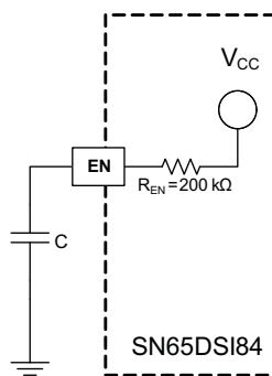
Figure 8. External Capacitor Controlled EN
