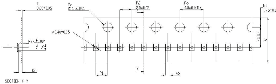
Device Orientation in Tape
