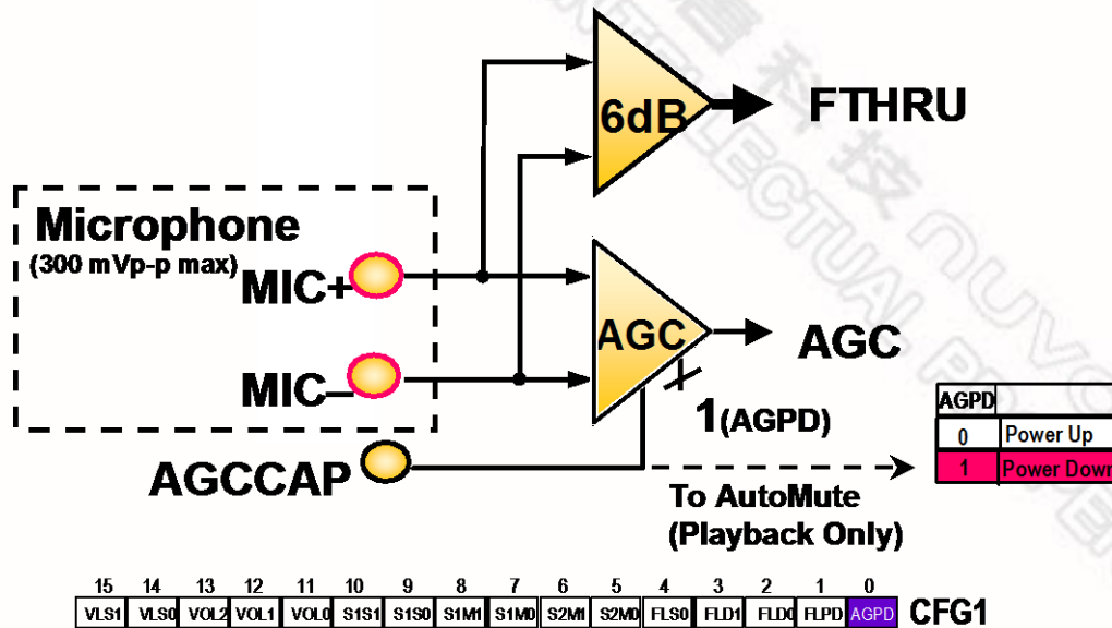
FIGURE 7: MICROPHONE AMPLIFIER
