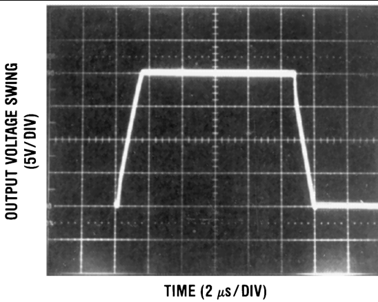
Figure 25. Large Signal Non-Inverting ( R_L = 2 \text{ k}\Omega , C_L = 10 \text{ pF} )
