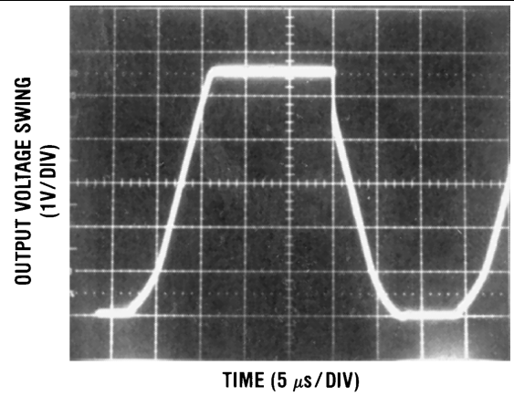
Figure 26. Current Limit ( R_L = 100\Omega ) ( C_L = 10 \text{ pF} )
