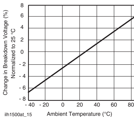
Fig. 16 - Switch Breakdown Voltage vs. Temperature
