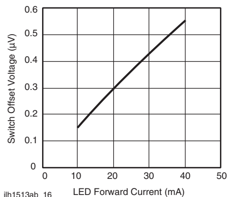
Fig. 17 - Switch Offset Voltage vs. LED Current
