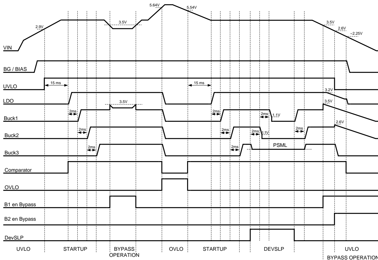
Figure 26. Operating Modes
