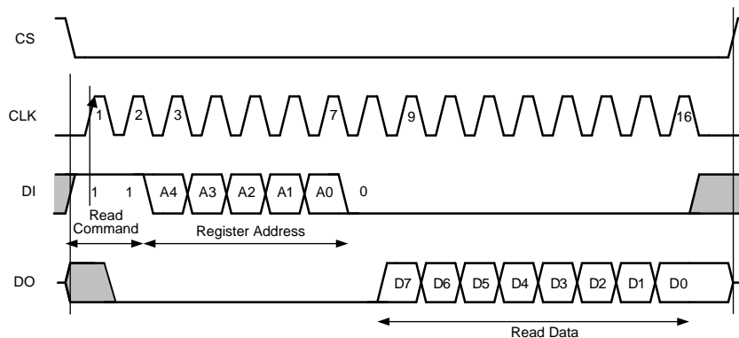
Figure 23. SPI Interface Read
