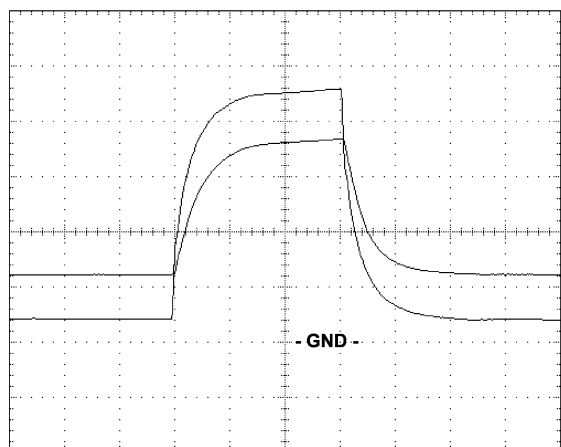
Figure 6. Logic Clamp Pulse
