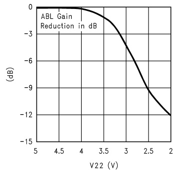
Figure 8. ABL Gain Reduction Curve
