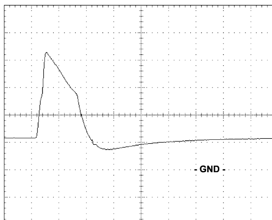
Figure 5. Deflection Vertical Blanking
