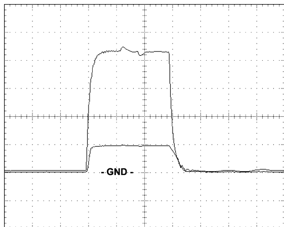
Figure 2. Logic Horizontal Blanking
