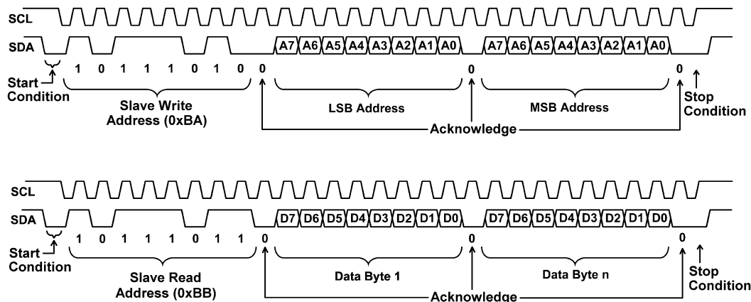
Figure 26. I 2 C Compatible Read Sequence
