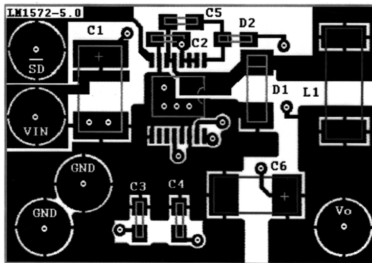
Figure 14. Top Layer
