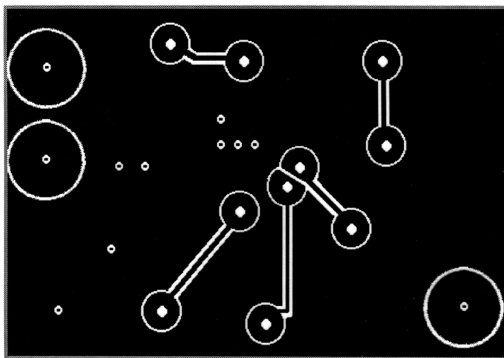
Figure 15. Bottom Layer
