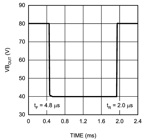
FIGURE 5. VB_{\text{OUT}} (40V P-P )
