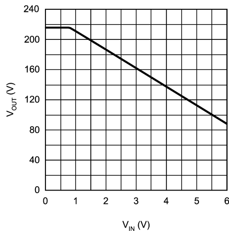
FIGURE 4. V_{\text{OUT}} vs. V_{\text{IN}}
