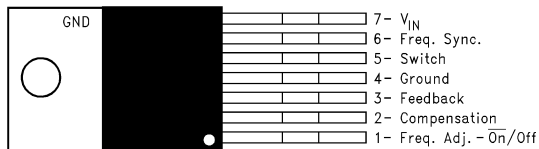
Figure 1. Bent, Staggered Leads 7-Lead TO-220 (NDZ) Top View See Package Number NDZ0007B
