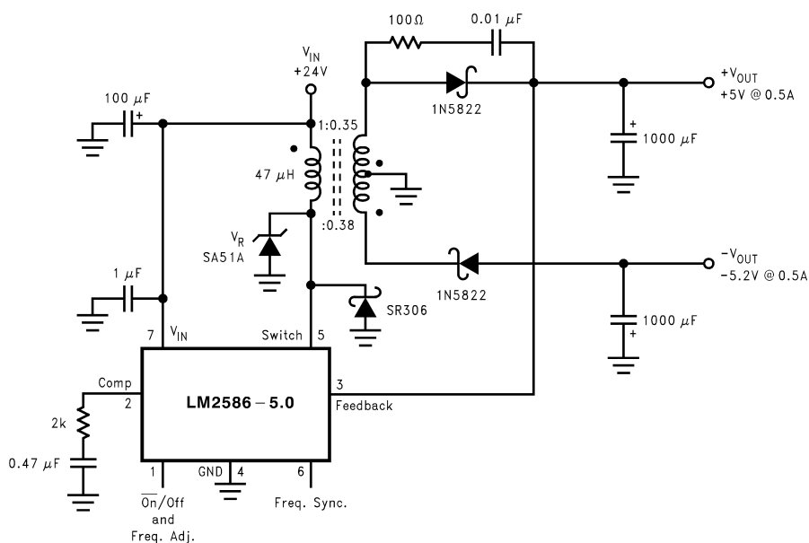
Figure 57. Flyback Regulator
