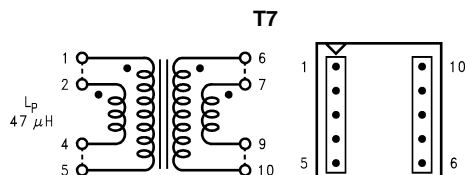
Figure 43. Schott 26606 (Top View)
