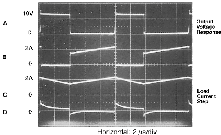
Figure 47. Switching Waveforms
