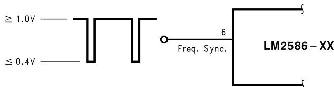
Figure 54. Frequency Synchronization
