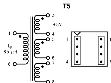
Figure 42. Renco RL-5532 (Top View)
