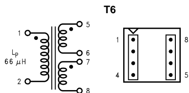
Figure 41. Renco RL-5533 (Top View)
