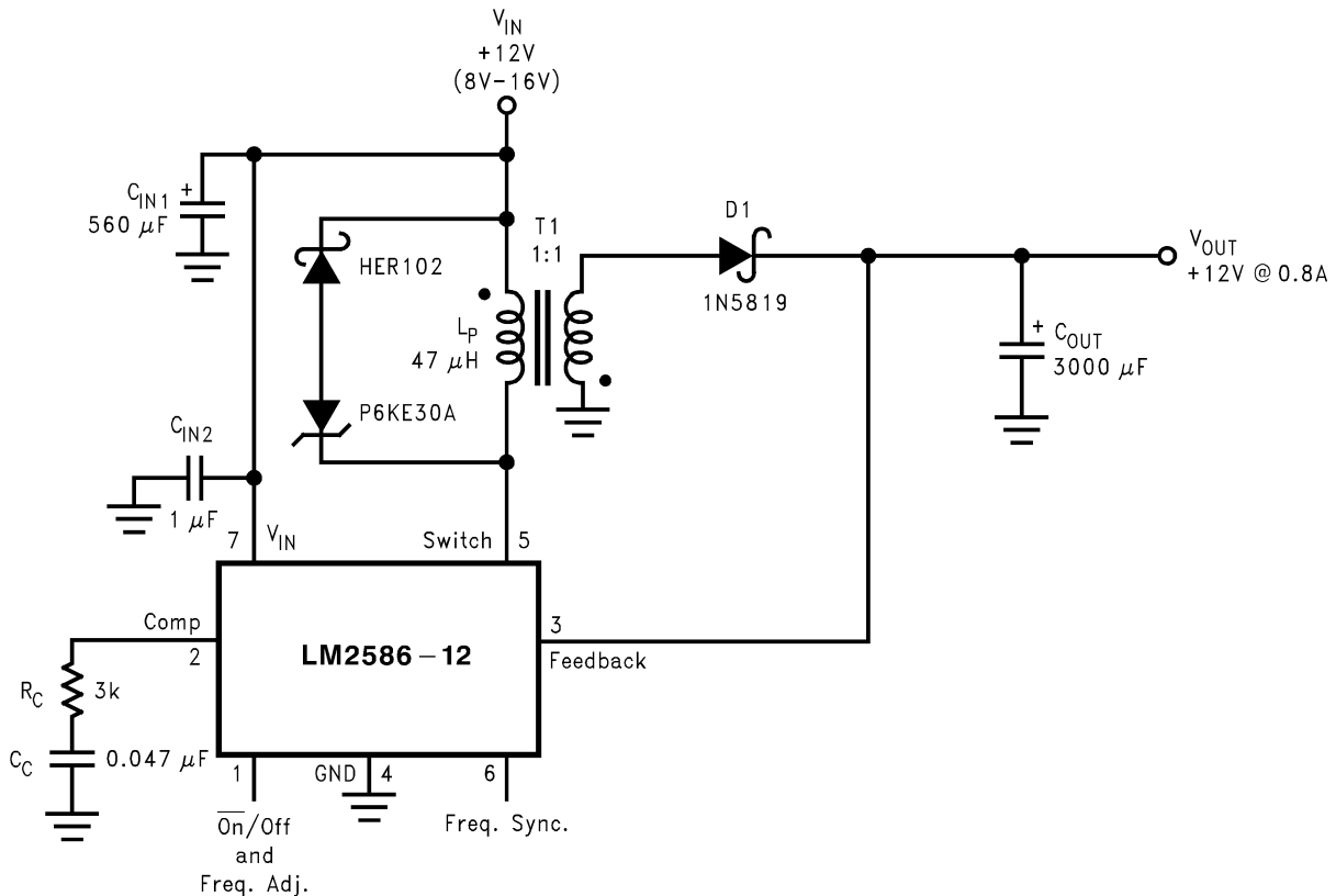
As shown in Figure 22, the LM2586 can be used as a flyback regulator by using a minimum number of external components. The switching waveforms of this regulator are shown in Figure 23. Typical Performance Characteristics observed during the operation of this circuit are shown in Figure 24.
