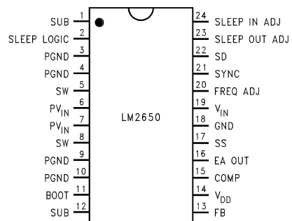
Figure 3. Top View 24-Lead Small Outline Package (DW) See Package Number DW0024B
