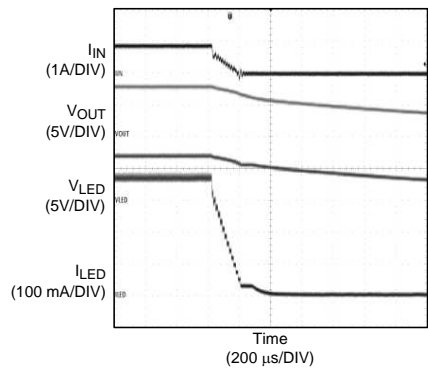
Ramp-Down 2 LEDs Simple Mode
