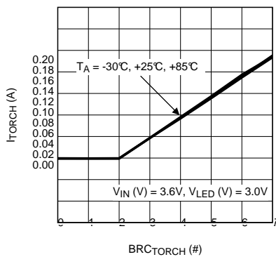
Torch Current vs Brightness Code 1 LED
