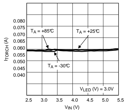
60mA Torch Current vs Input Voltage 1 LED
