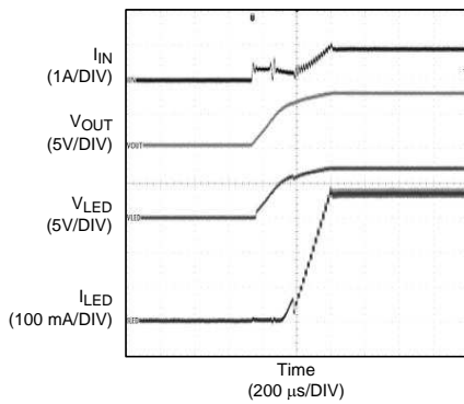
Startup 2 LEDs Simple Mode
