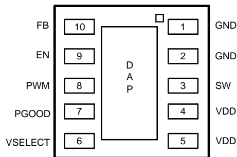
Figure 5. Bottom View
