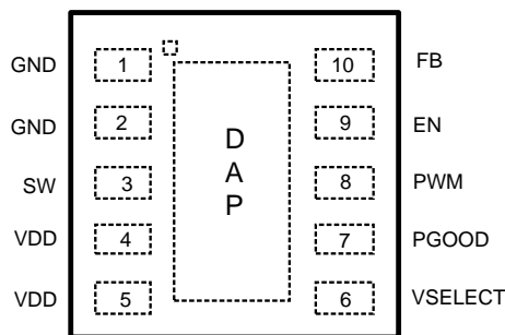
Figure 4. Top View
