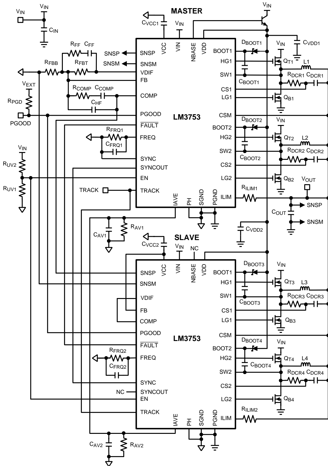
Figure 31. Typical Application
