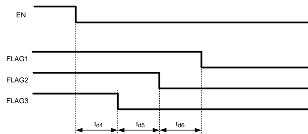
Figure 2. Power-Down Sequence
