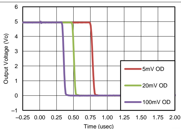
Figure 9. Response Time for Various Overdrives (Negative Transition)
