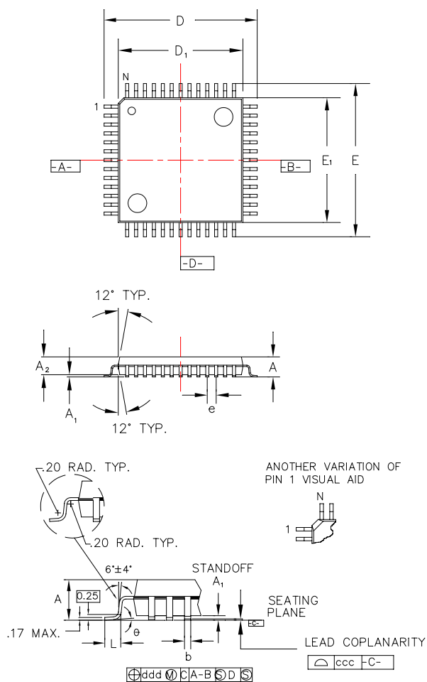
Figure C-1. Stellaris LM3S1651 100-Pin LQFP Package Dimensions
