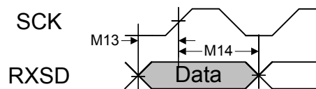
Figure 23-19. I 2 S Master Mode Receive Timing
