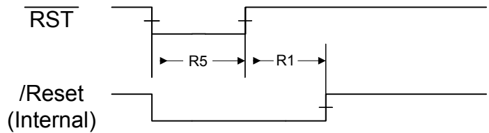
Figure 23-7. External Reset Timing ( \overline{\text{RST}} )
