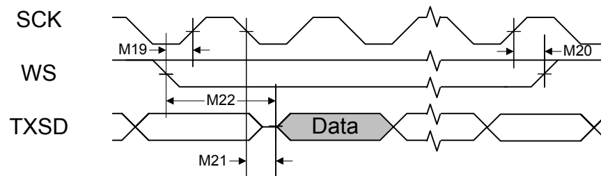
Figure 23-20. I 2 S Slave Mode Transmit Timing
