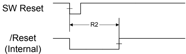
Figure 23-8. Software Reset Timing
