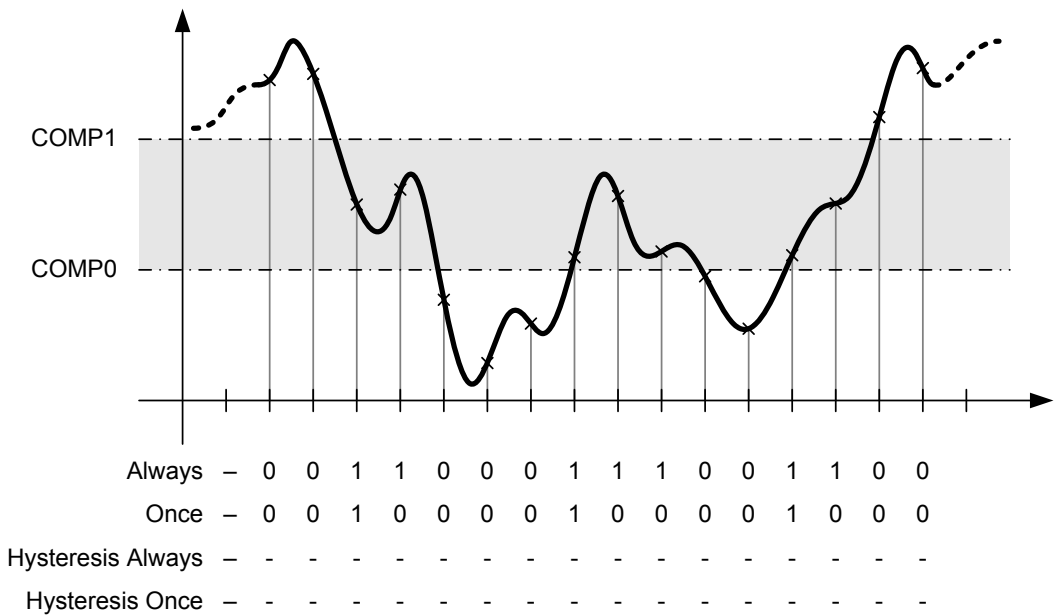
Figure 13-15. Mid-Band Operation (CIC=0x1 and/or CTC=0x1)
