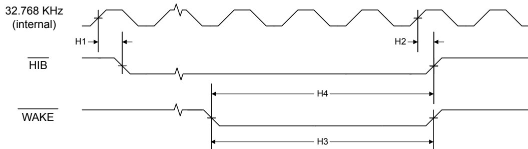
Figure 20-9. Hibernation Module Timing
