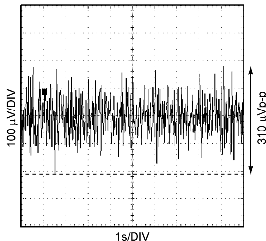
Figure 38. 0.1–10 Hz Noise
