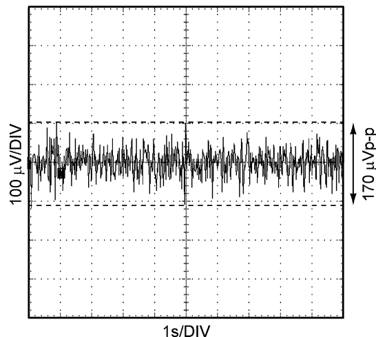
Figure 14. 0.1–10 Hz Noise
