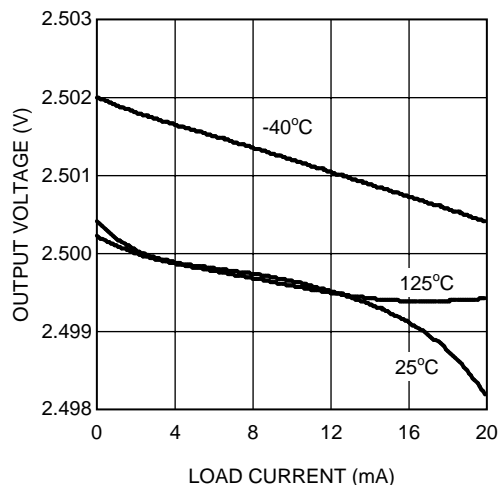
Figure 24. Load Regulation
