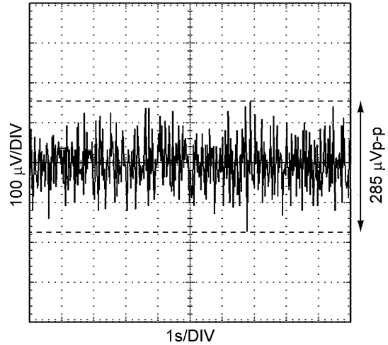
Figure 32. 0.1–10 Hz Noise
