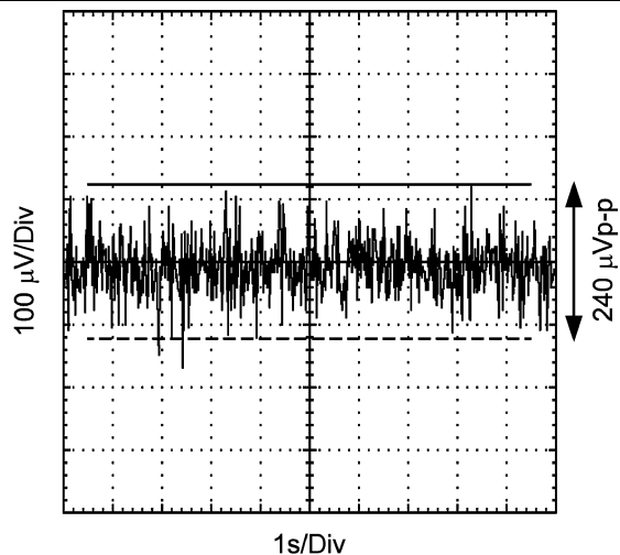
Figure 26. 0.1–10 Hz Noise
