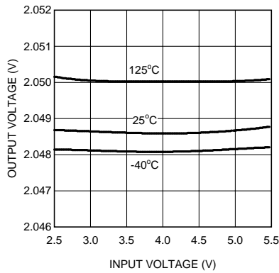
Figure 9. Line Regulation
