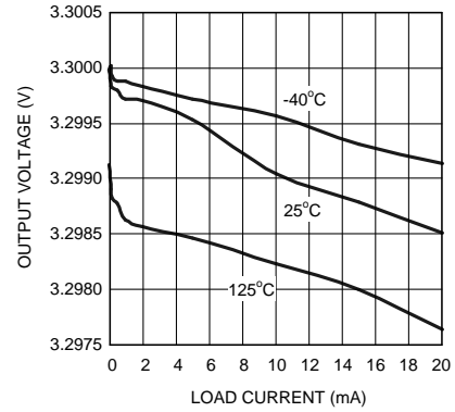
Figure 26. Load Regulation
