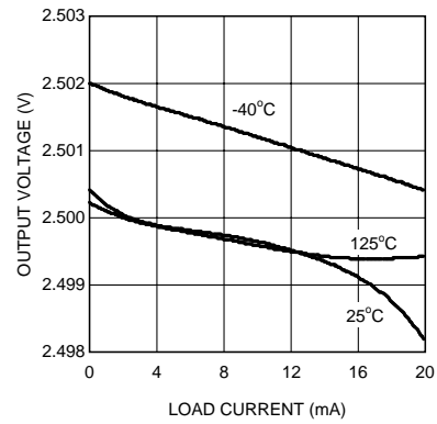
Figure 14. Load Regulation
