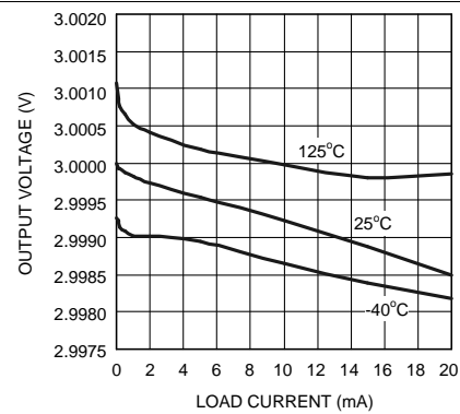
Figure 20. Load Regulation
