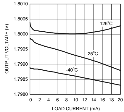
Figure 2. Load Regulation
