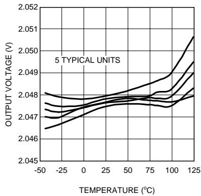
Figure 7. Output Voltage vs Temperature
