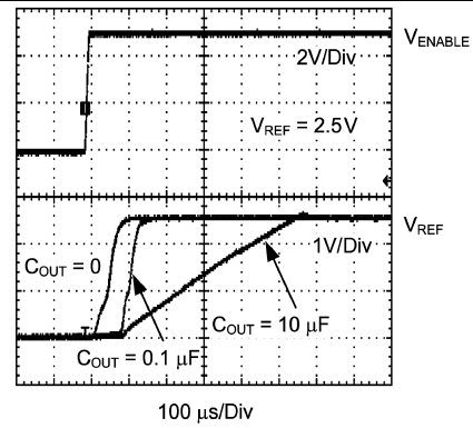
Figure 44. Turn-On Transient Response
