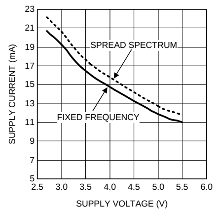
Figure 16. Supply Current vs Supply Voltage PV_1 = 7 \text{ V}
