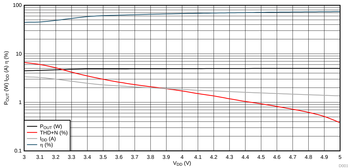
Figure 24. V_{DD} vs P_{OUT} , I_{DD} , and Efficiency With 4-Ω Load
