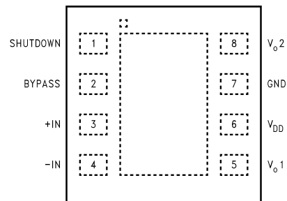
Figure 3. WSO8 - Top View See Package Number NGL
