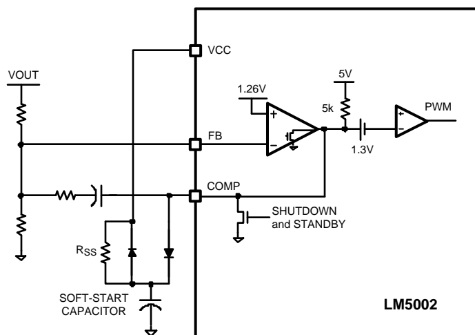
Figure 20. Soft-Start
