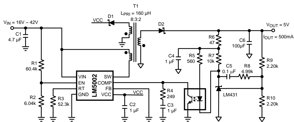
Figure 22. Isolated Flyback
