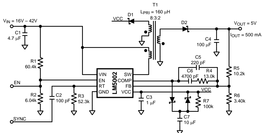
Figure 21. Non-Isolated Flyback
