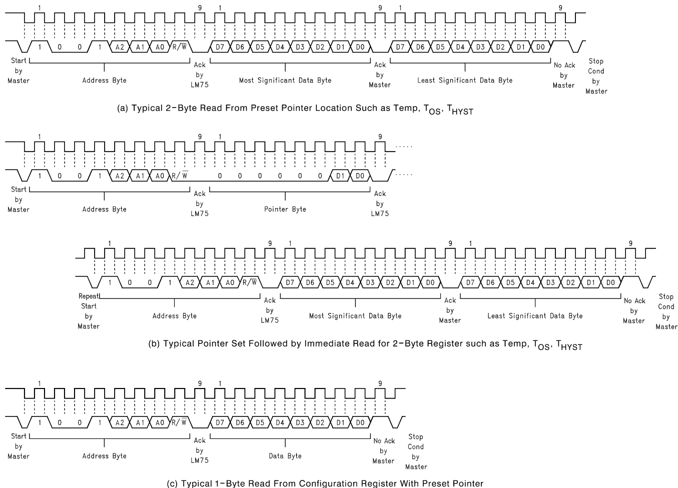
Figure 4. I²C Timing Diagrams
