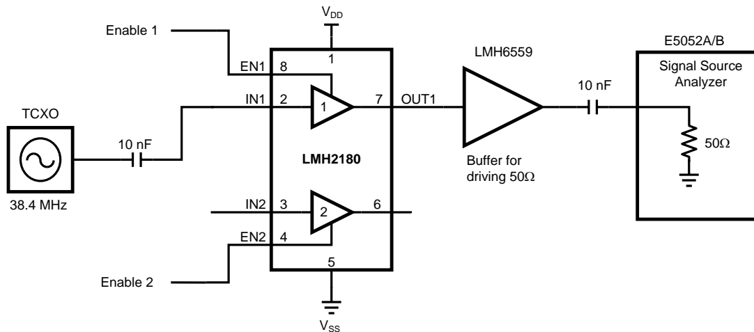
Figure 40. Measurement Setup
