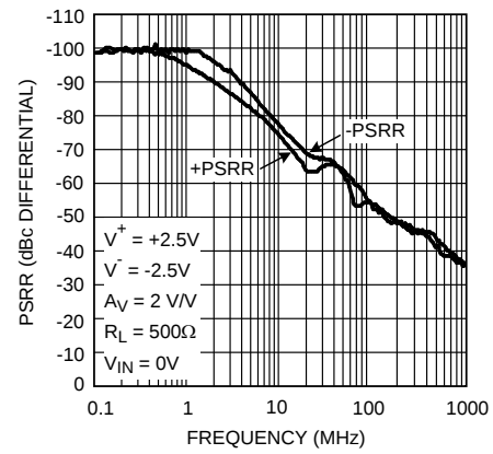
Figure 28. PSRR
