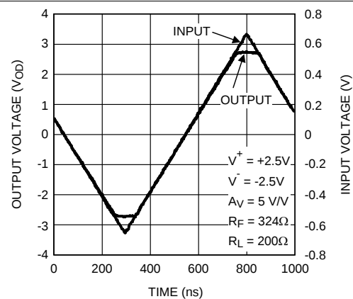
Figure 26. Overdrive Recovery
