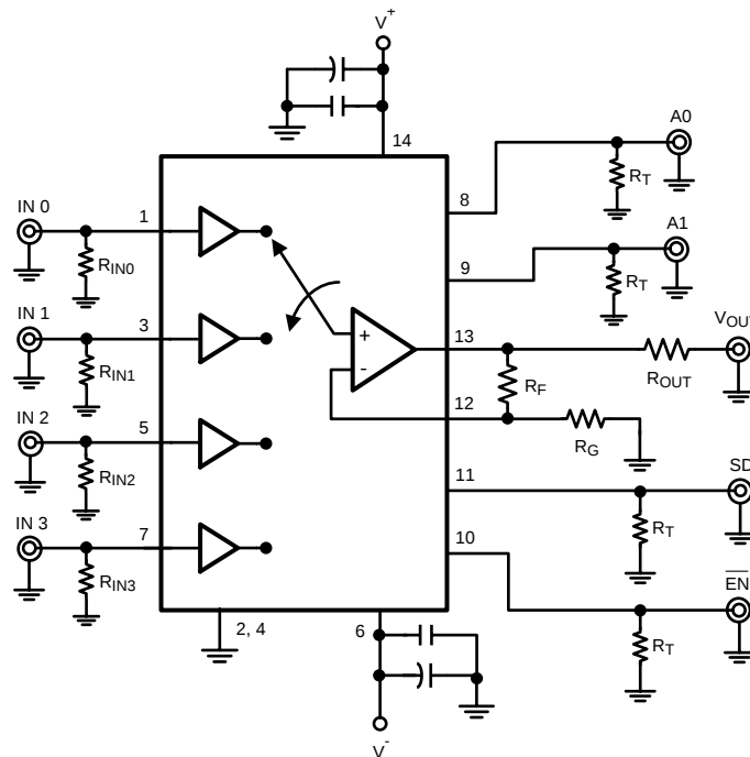
Figure 27. Typical Application
