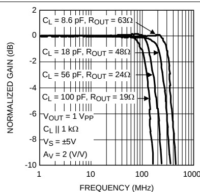
Figure 34. Decoupling Capacitive Loads
