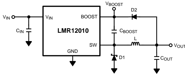
Figure 22. V_{OUT} Charges C_{BOOST}
