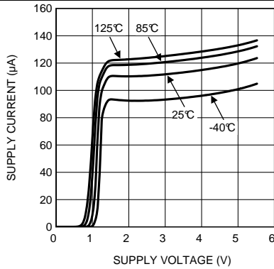
Figure 1. Supply Current vs. Supply Voltage (LMV931-N)
