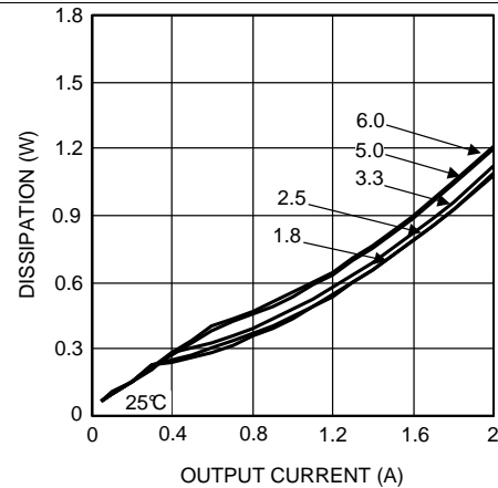
Figure 10. Dissipation 12-V Input at 25°C
