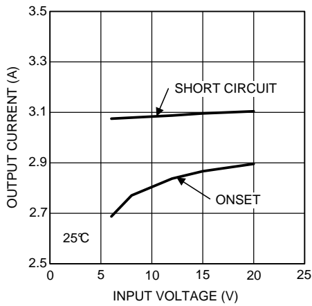
Figure 31. Current Limit 3.3 V_{OUT} at 25°C
