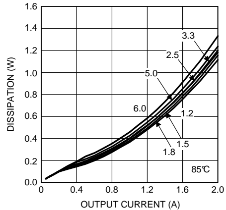
Figure 20. Dissipation 8-V Input at 85°C
