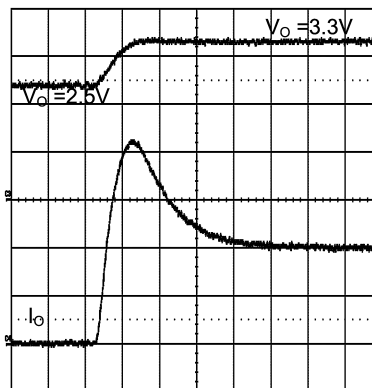
Figure 35. Prebiased Start-Up
