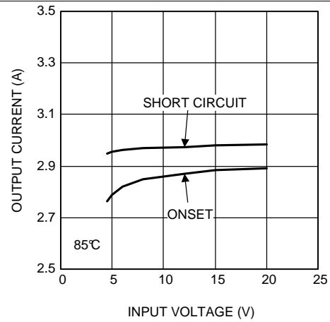
Figure 32. Current Limit 1.8 V_{OUT} at 85°C
