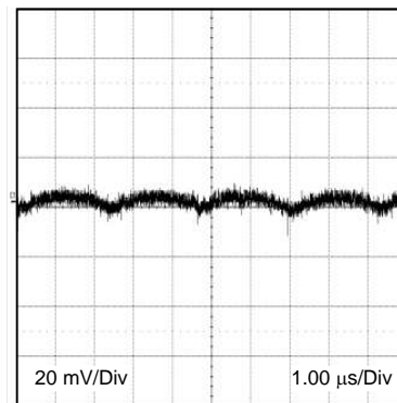
12 V_{IN} 3.3 V_O 2 A 20 mV/div 1 \mu\text{s/div}
