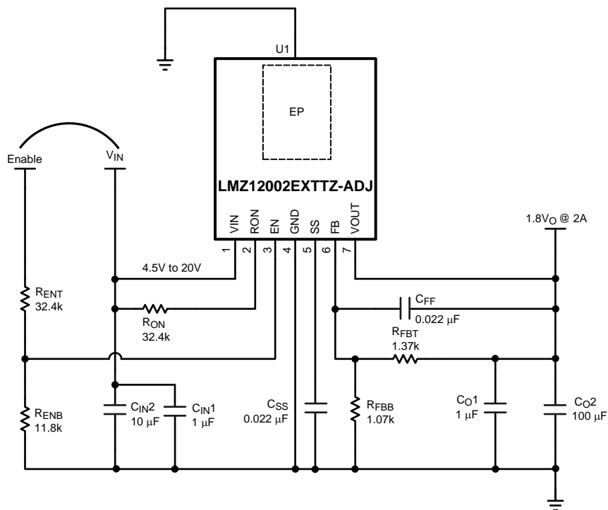
Figure 36. Evaluation Board Schematic Diagram
