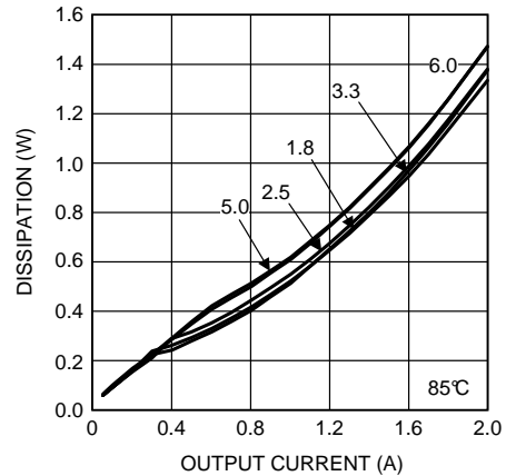
Figure 22. Dissipation 12-V Input at 85°C
