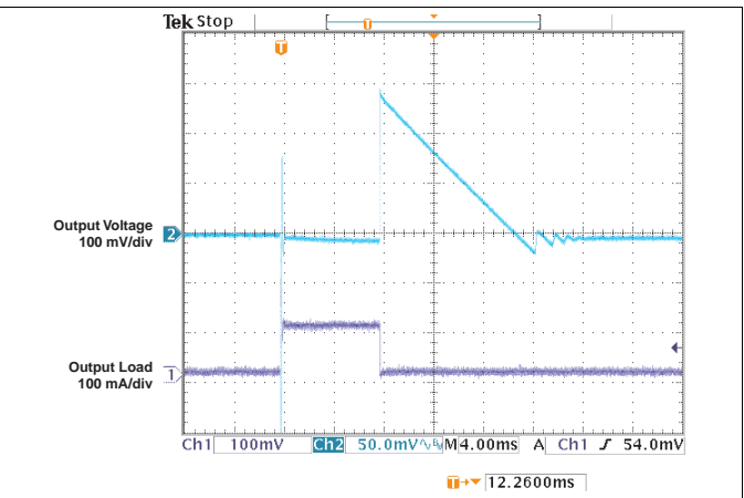
Figure 20. Load Transient Response vs Time ( V_{OUT} = 5\text{ V} , C_L = 10\ \mu\text{F} )
