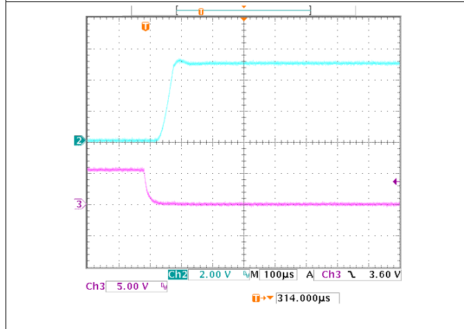
Figure 21. Enable Transient Response vs Time ( C_L = 1\ \mu\text{F} , I_L = 1\ \text{mA} )
