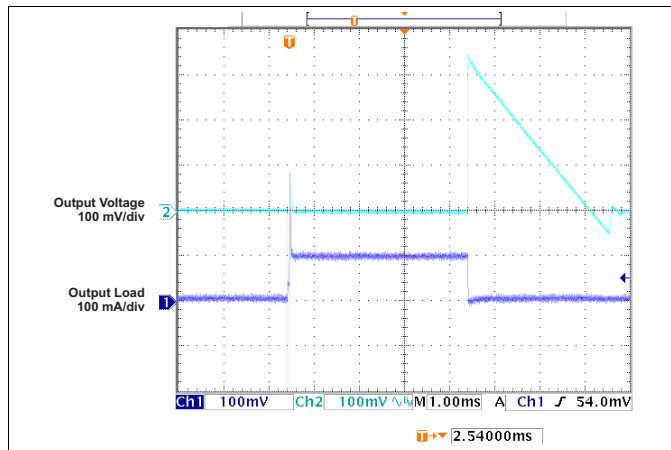
Figure 19. Load Transient Response vs Time ( V_{OUT} = 5\text{ V} , C_L = 1\ \mu\text{F} )
