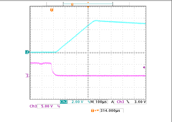
Figure 22. Enable Transient Response vs Time ( C_L = 10\ \mu\text{F} , I_L = 1\ \text{mA} )
