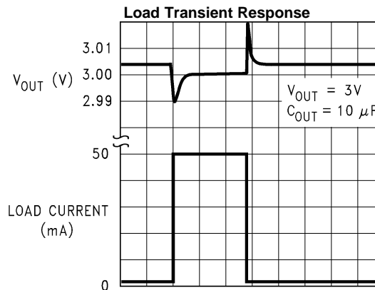
10 \mu\text{s}/\text{div} \rightarrow Figure 17.
