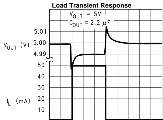
10 \mu\text{s}/\text{div} \rightarrow Figure 18.
