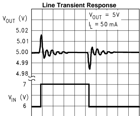
20 \mu\text{s}/\text{div} \rightarrow Figure 14.
