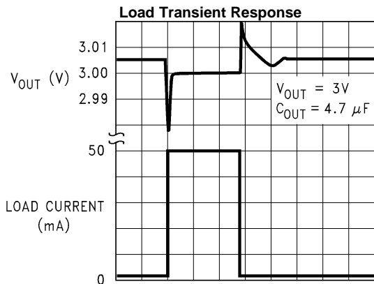
10 \mu\text{s}/\text{div} \rightarrow Figure 16.
