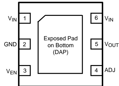
Figure 3. 6-Lead WSON (LP38692SD-ADJ) Top View See Package Number NGG
