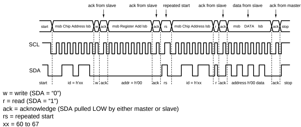
Figure 6. LP3943 Register Read
