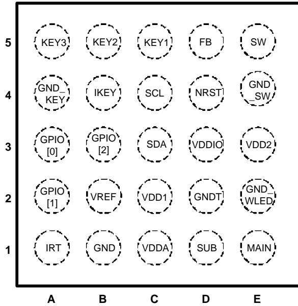
Figure 1. Top View
