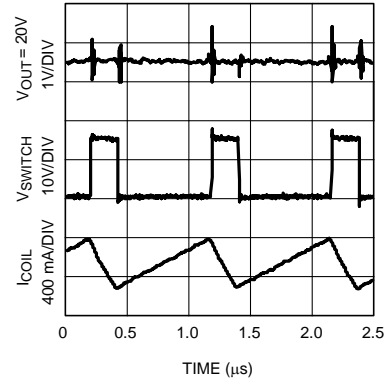
Figure 18. Boost Typical Waveforms at 60 mA Load
