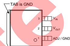
DD PACKAGE (Top View)
