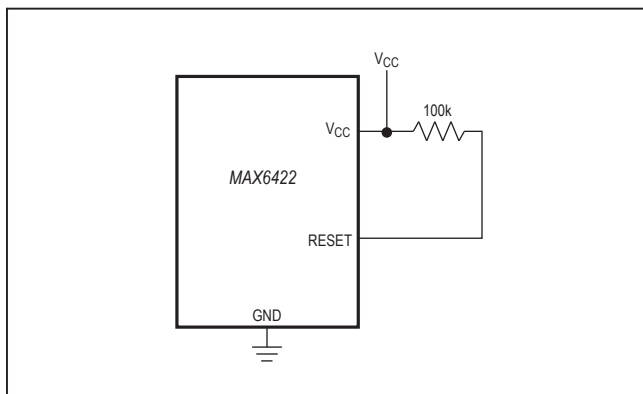
Figure 4. Ensuring \text{RESET} Valid to V_{CC} = 0
