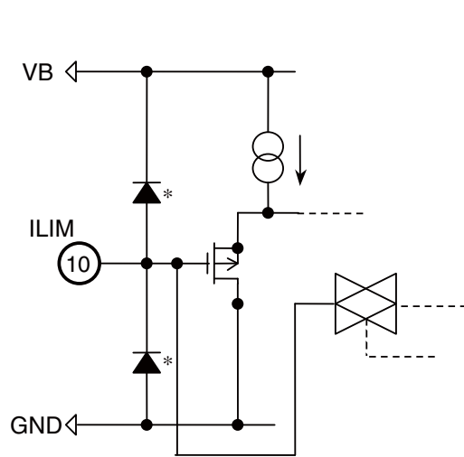
<<Over current detection block>>
