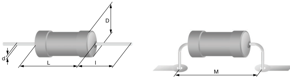
DIMENSIONS - Leded resistor types, mass and relevant physical dimensions
