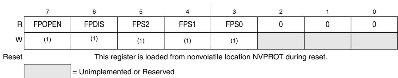
Figure 4-8. FLASH Protection Register (FPROT)
