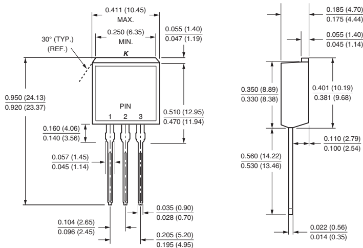
TO-262AA
