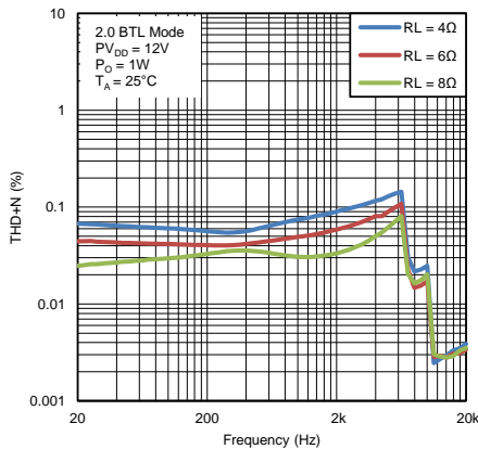
Figure 22. Total Harmonic Distortion vs Frequency (2.0 BTL Mode)
