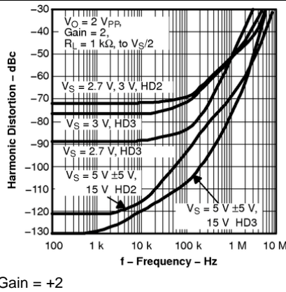
Figure 43. Harmonic Distortion vs Frequency
