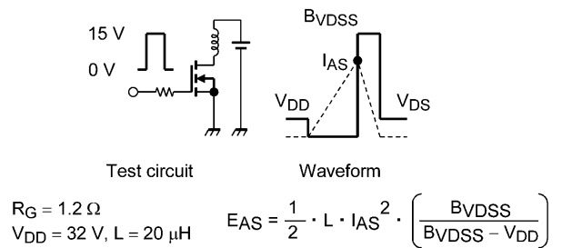
Fig. 8.15 Test Circuit/Waveform
