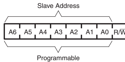
Figure 17. Slave Address
