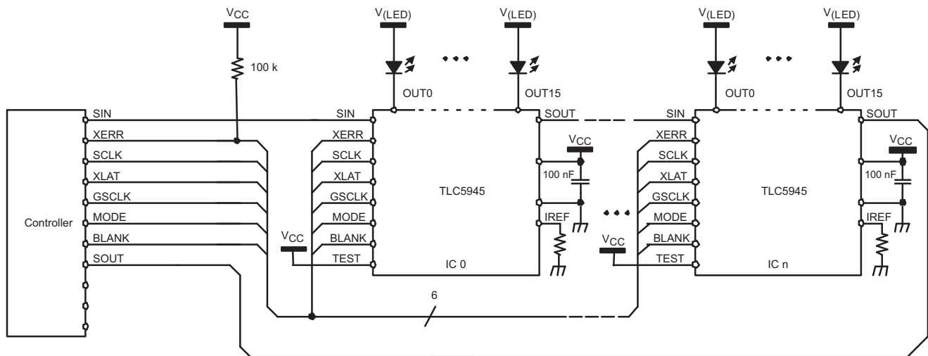
Figure 16. Cascading Devices
